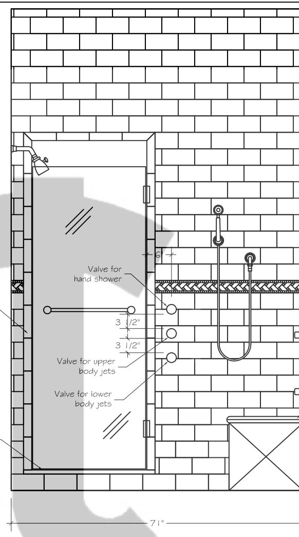
3 MASTER BATH SHOWER SCALE: 1/2" = 1'-0"
