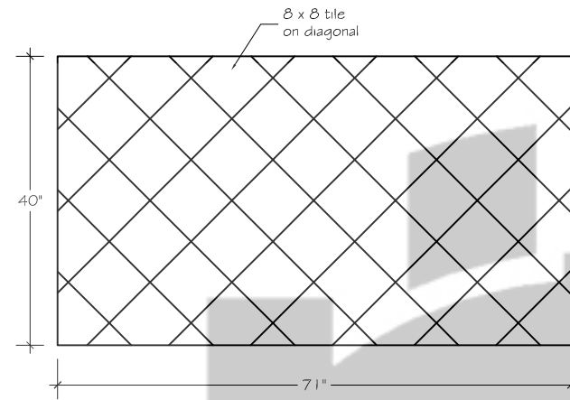
2 MASTER BATH SHOWER - CEILING SCALE: 1/2" = 1'-0"
