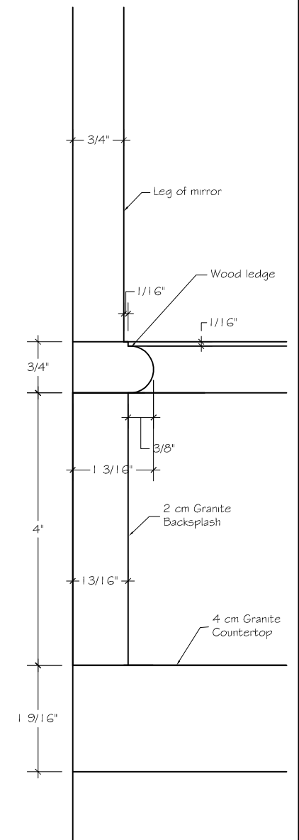
5 MASTER BATH DETAIL SCALE: HALF
