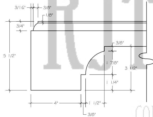
6 TYPICAL BASE DETAIL SCALE: 3" = 1'-0"
