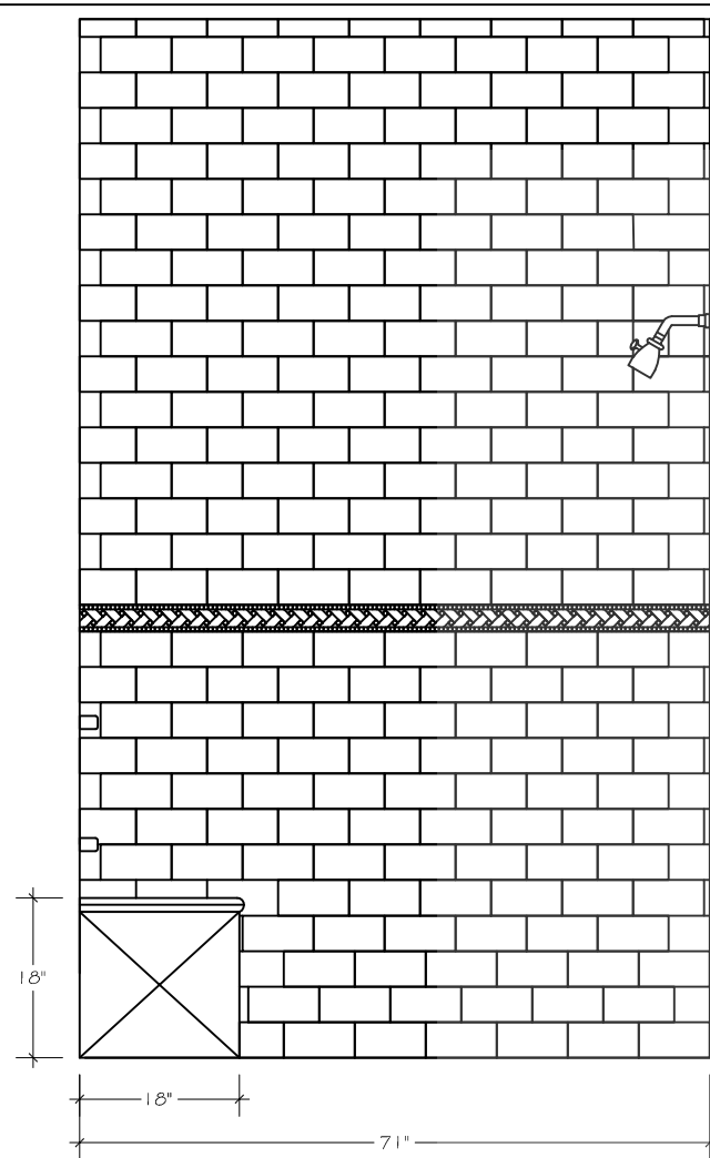
1 MASTER BATH SHOWER SCALE: 1/2" = 1'-0"
