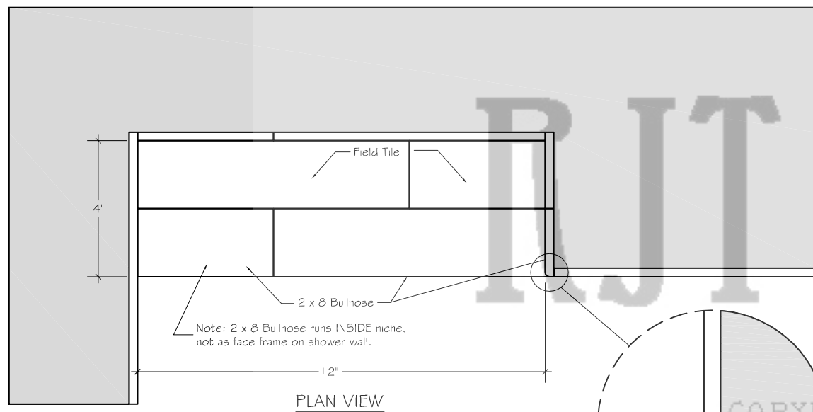
6 SHOWER NICHE DETAIL SCALE: 3" = 1'-0"
