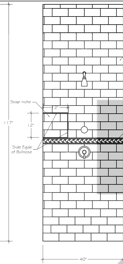
2 MASTER BATH SHOWER SCALE: 1/2" = 1'-0"
