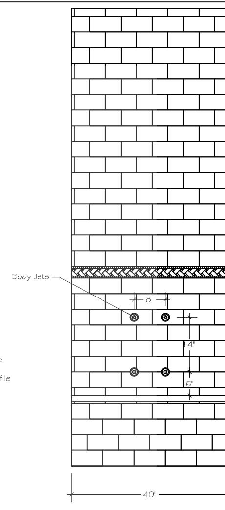
4 MASTER BATH SHOWER SCALE: 1/2" = 1'-0"
